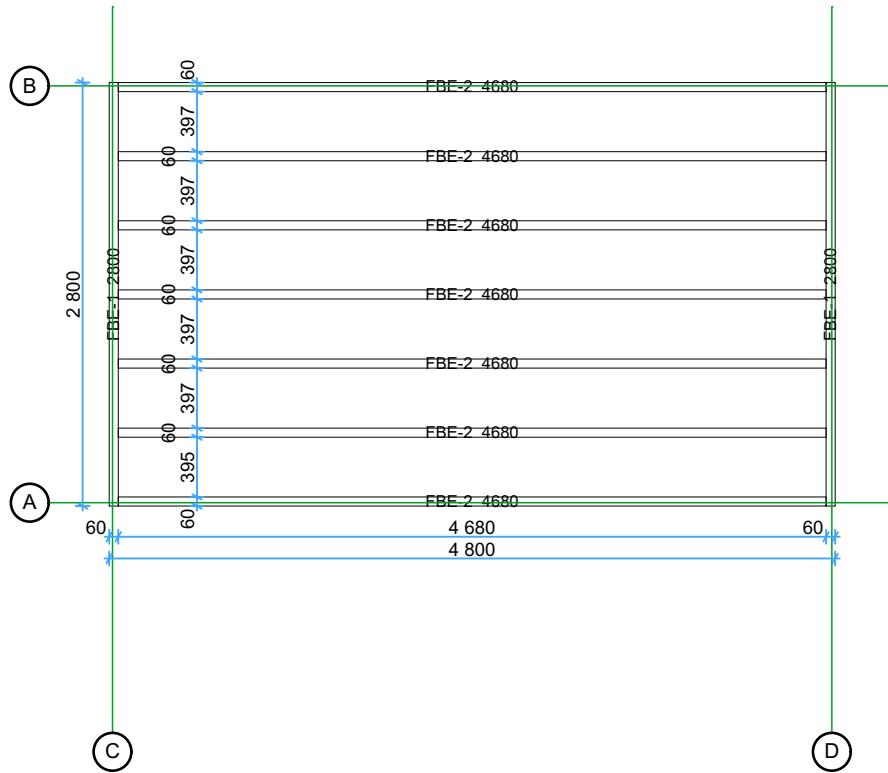
Floor bearer
