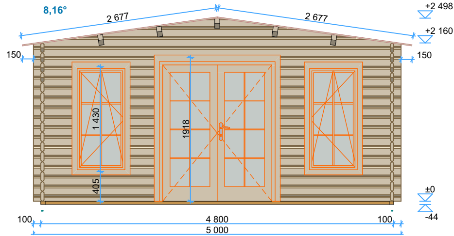
Back Elevation
