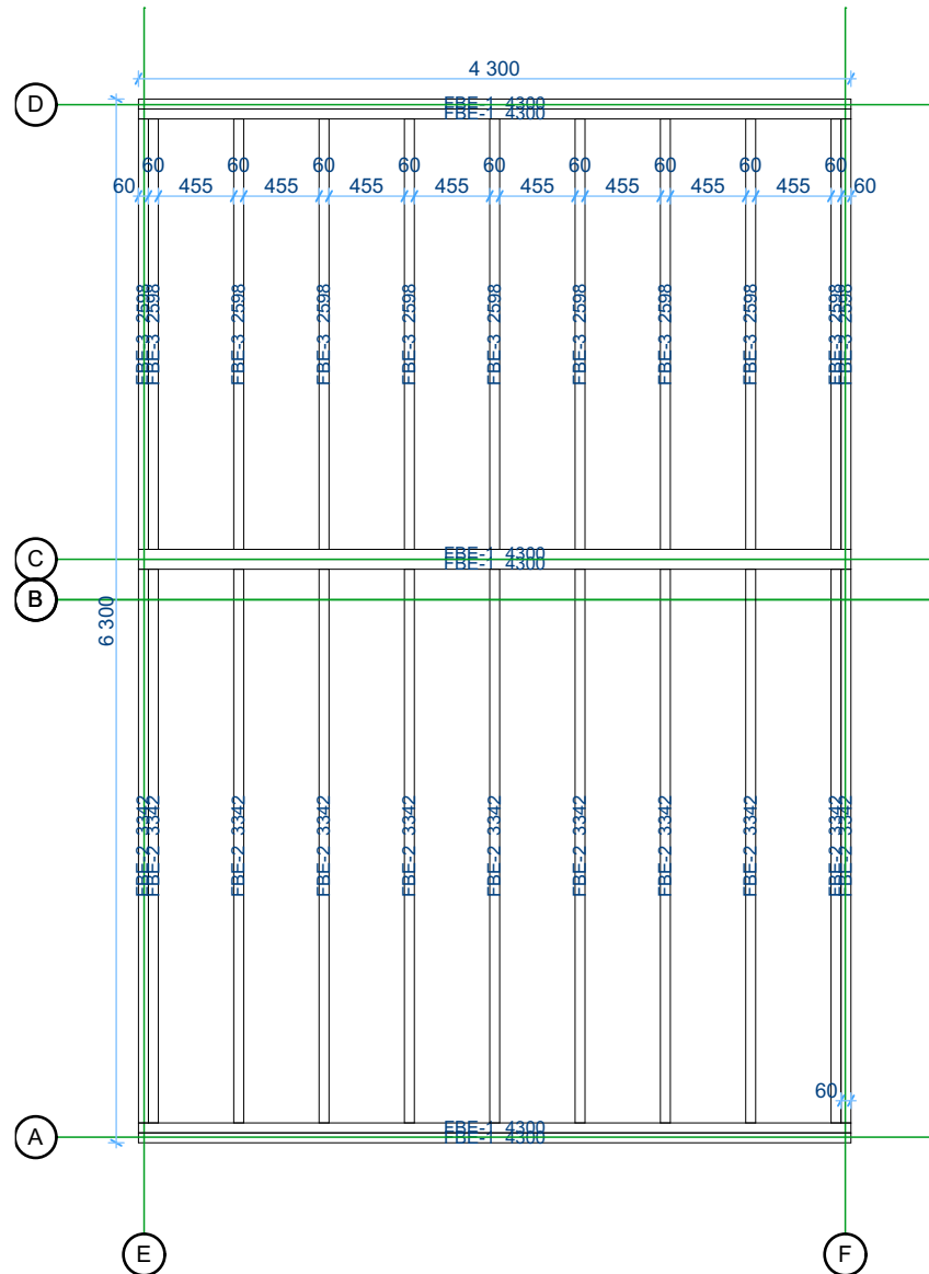
Floor bearers 1:50
