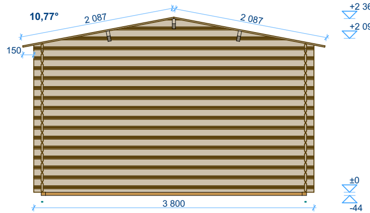
Back Elevation
