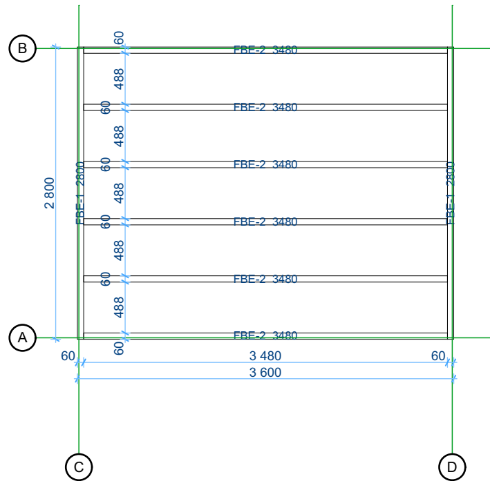
Floor bearers plan
