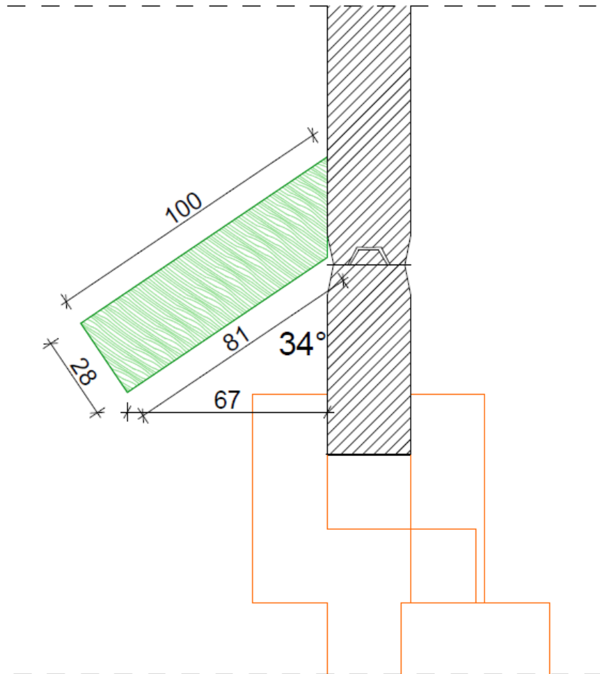
Drip cap over window/door
