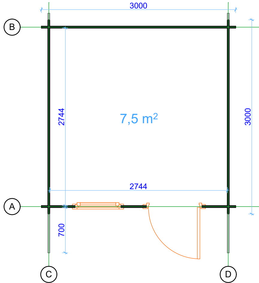
Floor plan
