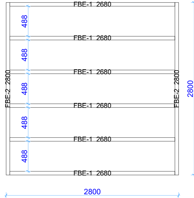
Floor bearers
