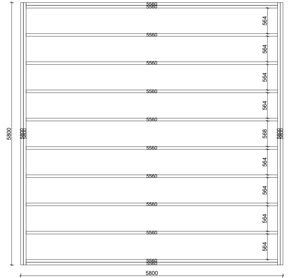
Floor bearers 1:50
