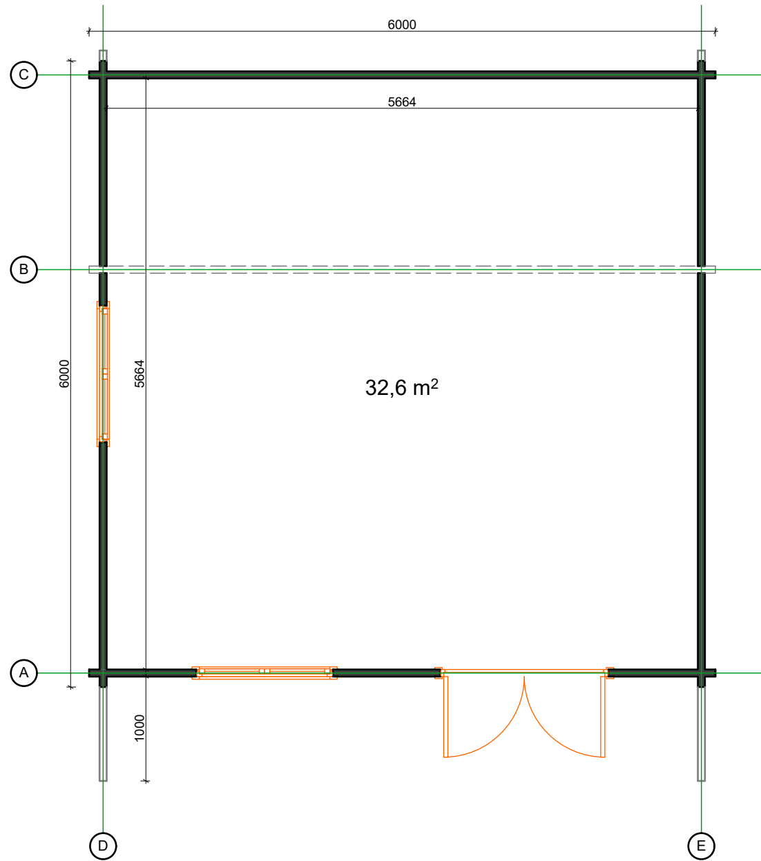
Floor plan 1:50
