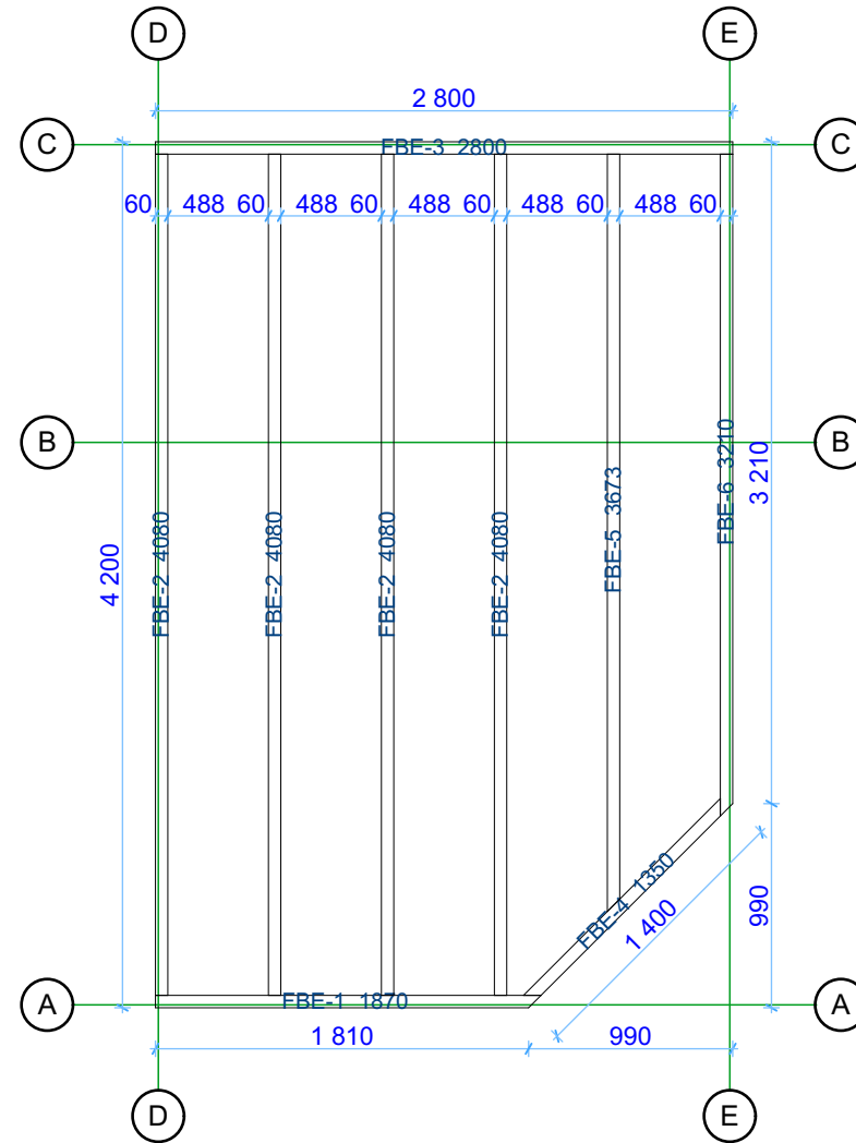
Floor bearers
