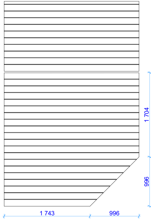
Floor boards 1:40
