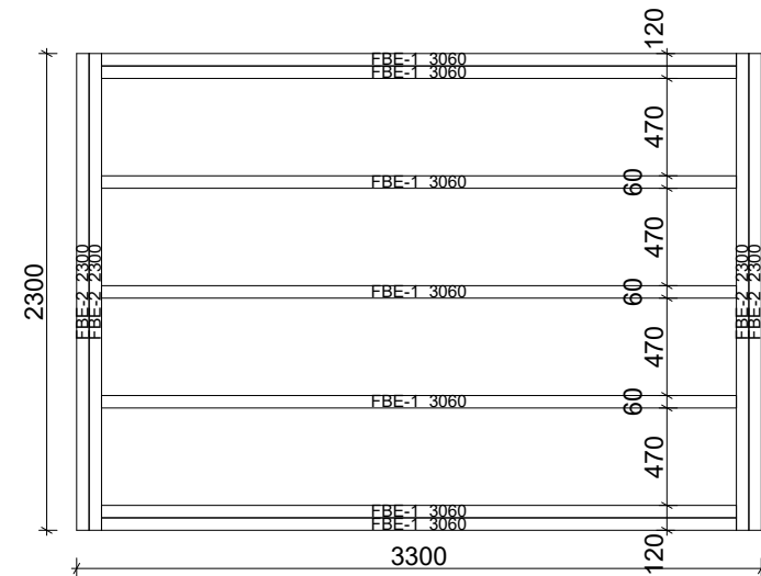
Floor bearers 1:40
