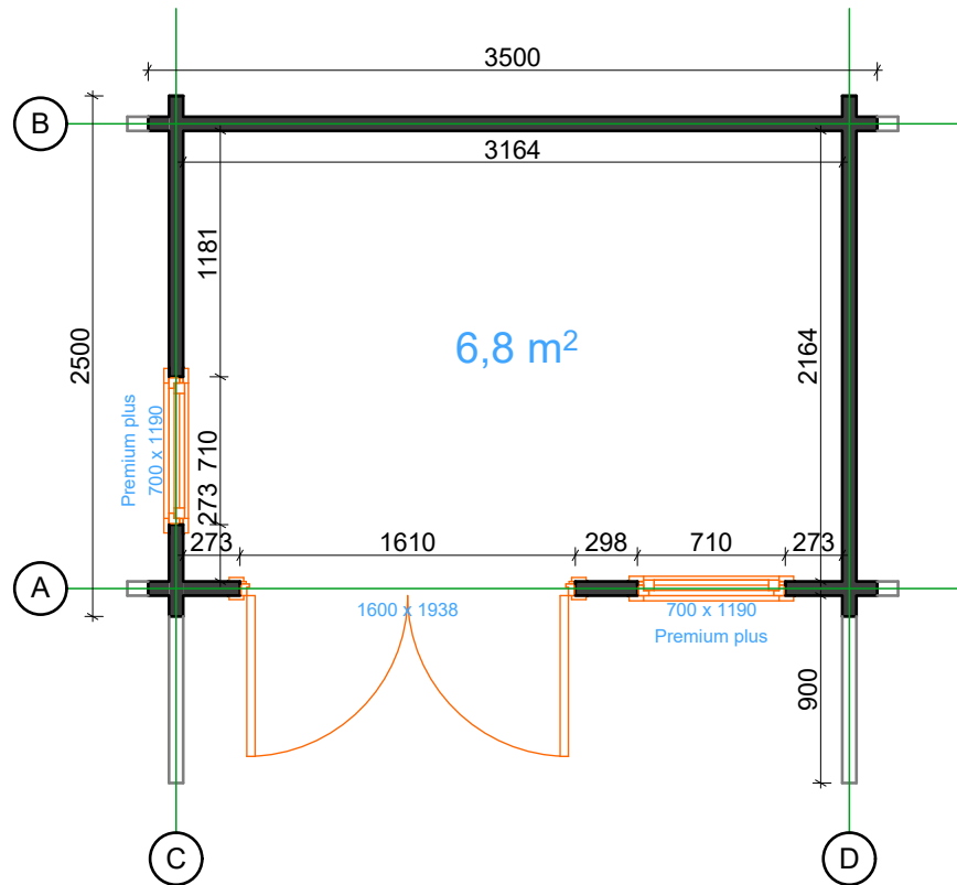
Floor plan 1:40
