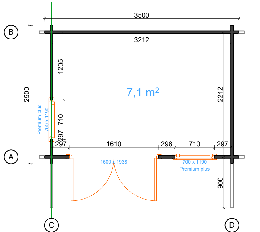
Floor plan 1:40
