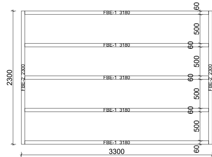
Floor bearers 1:40
