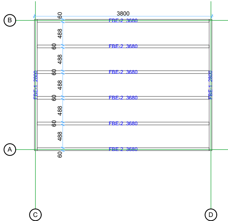
Floor bearers 1:50
