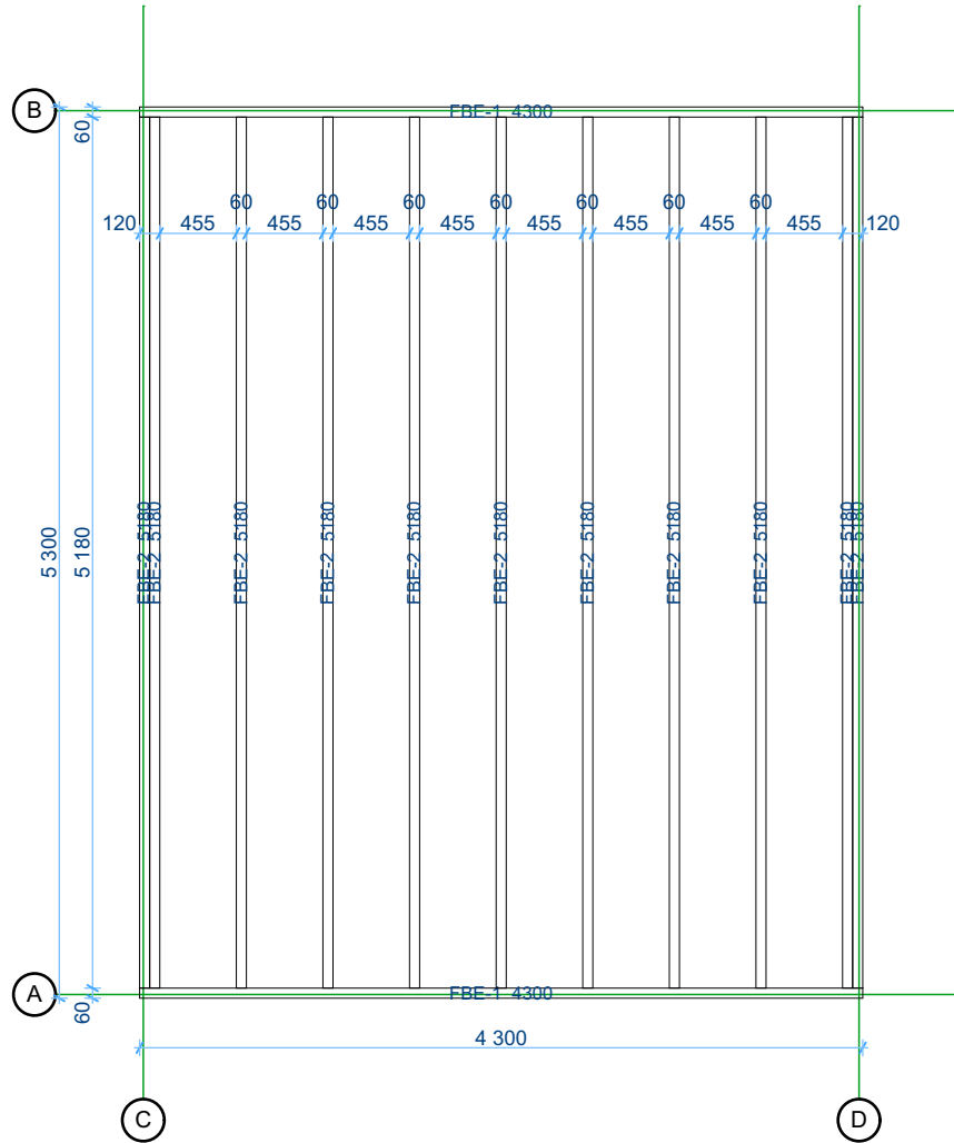
Floor bearers plan
