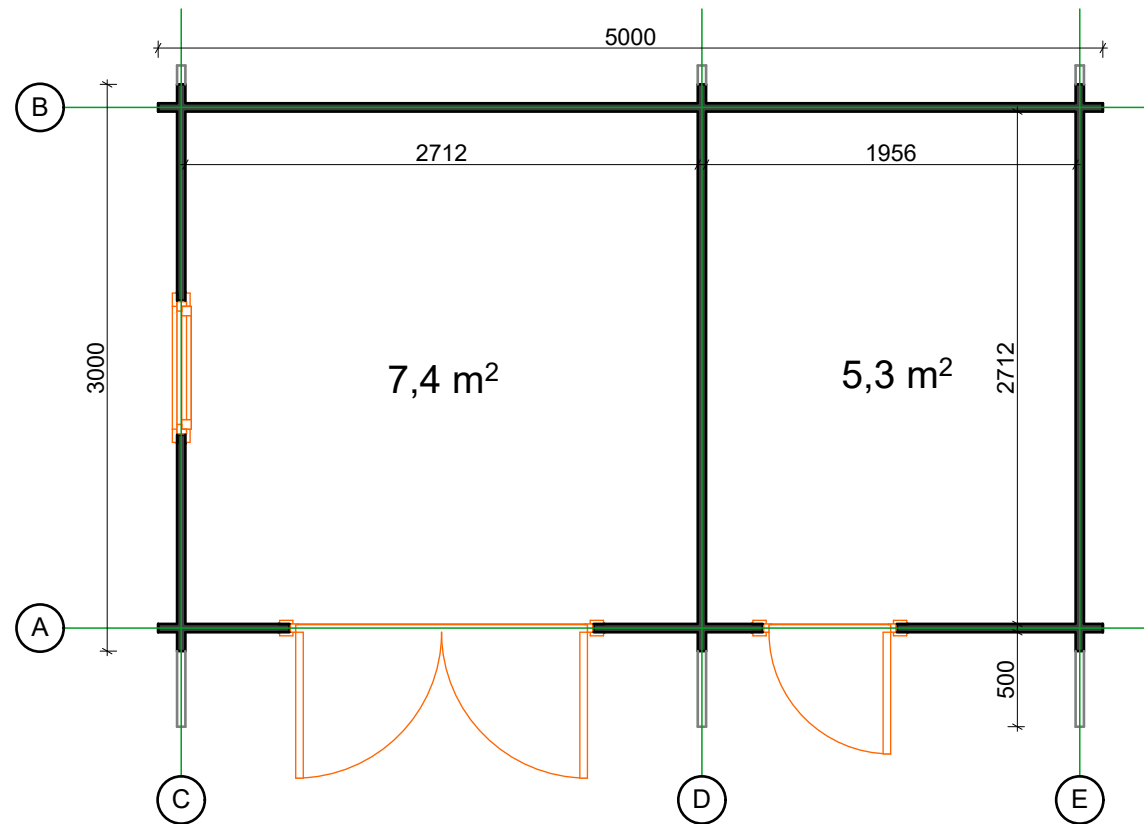
Floor plan 1:40
