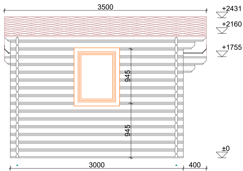
Left view
